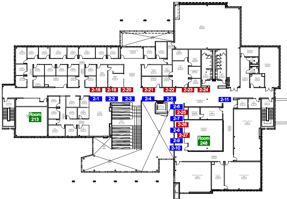
KNOWLTON CENTER - SECOND FLOOR PLAN
